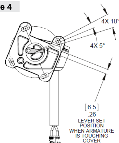
BEFORE ENERGIZING ACTUATOR
